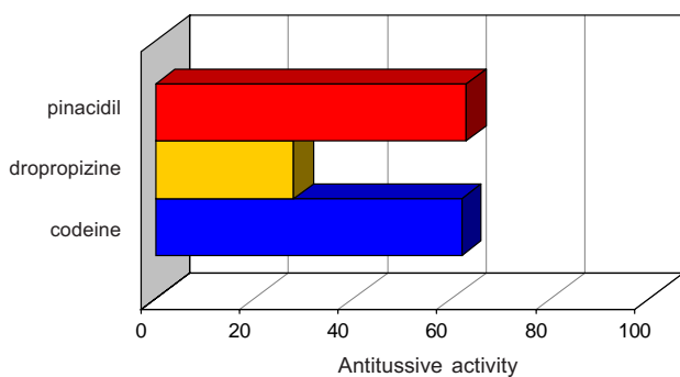
Fig. 4. Antitussive activity (in %) of pinacidil (expressed according to NE, IA^+ and IA^- ) in comparison to reference drugs (codeine, dose 10 \text{ mg.kg}^{-1} b.w. intraperitoneally and dropropizine, dose 30 \text{ mg.kg}^{-1} b.w. intraperitoneally) on mechanically induced cough in conscious cats.
